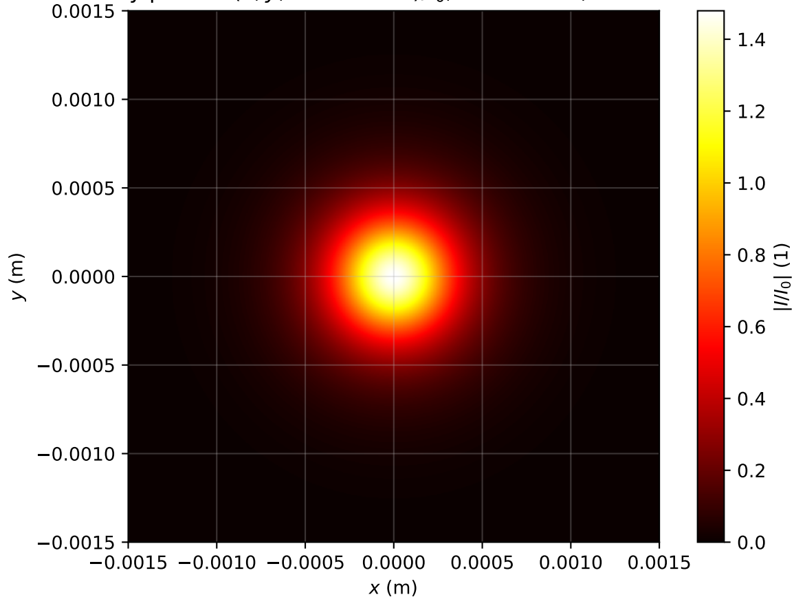
Intensity profile I(x, y, z = 1.194m)/I_0 , \text{Pin}=0.9\text{Pcr} , artificial time
